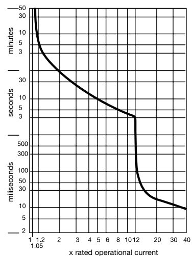
Cold state curve. For warm state multiply t x 0,25
